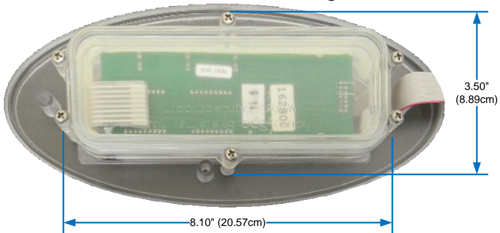
Bottom View for Hole Through Shell
